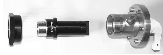
Aircraft Sampling System
